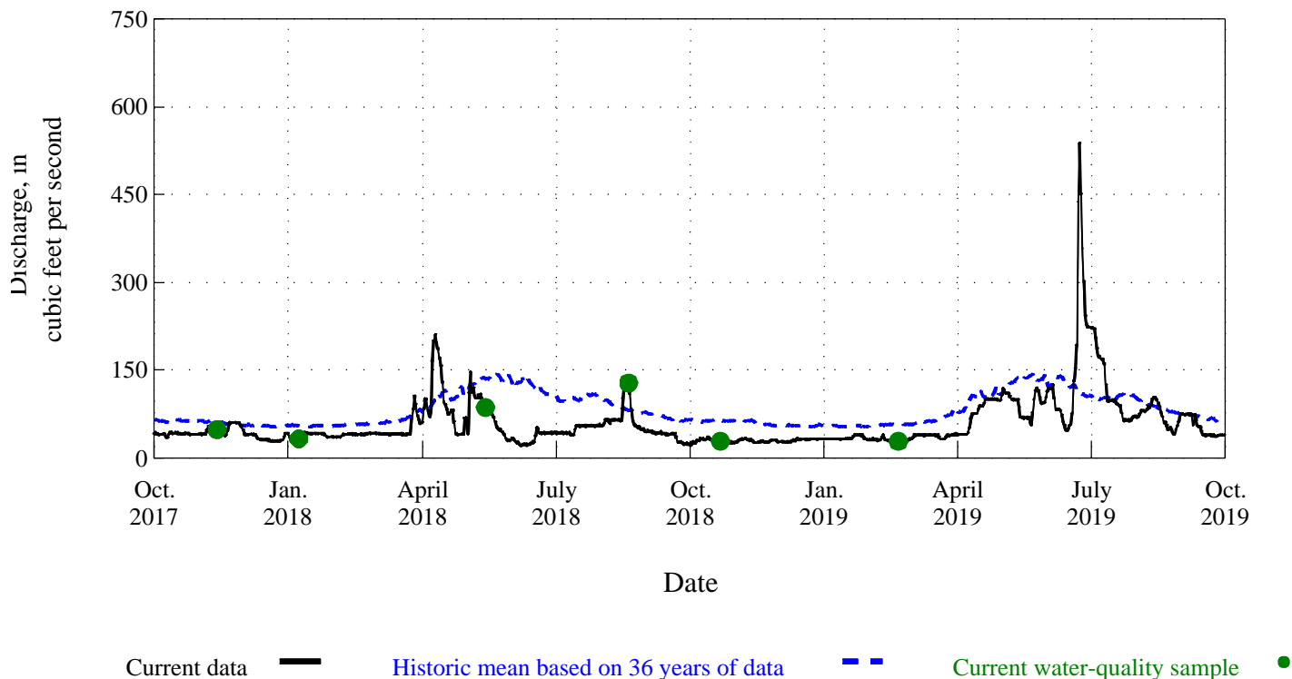
Figure 5. Time distribution and associated discharge of water-quality samples for Yampa River below Stagecoach Reservoir, Co., station 09237500.
