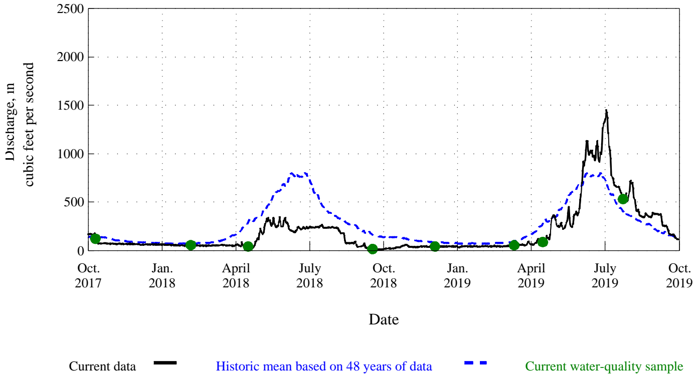
Figure 7. Time distribution and associated discharge of water-quality samples for Uncompahgre River at Colona, CO, station 09147500.
