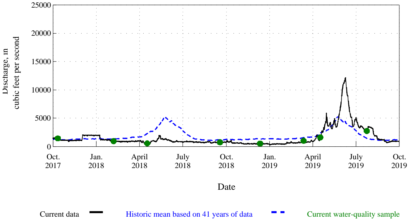
Figure 16. Time distribution and associated discharge of water-quality samples for Gunnison River at Delta, CO, station 09144250.
