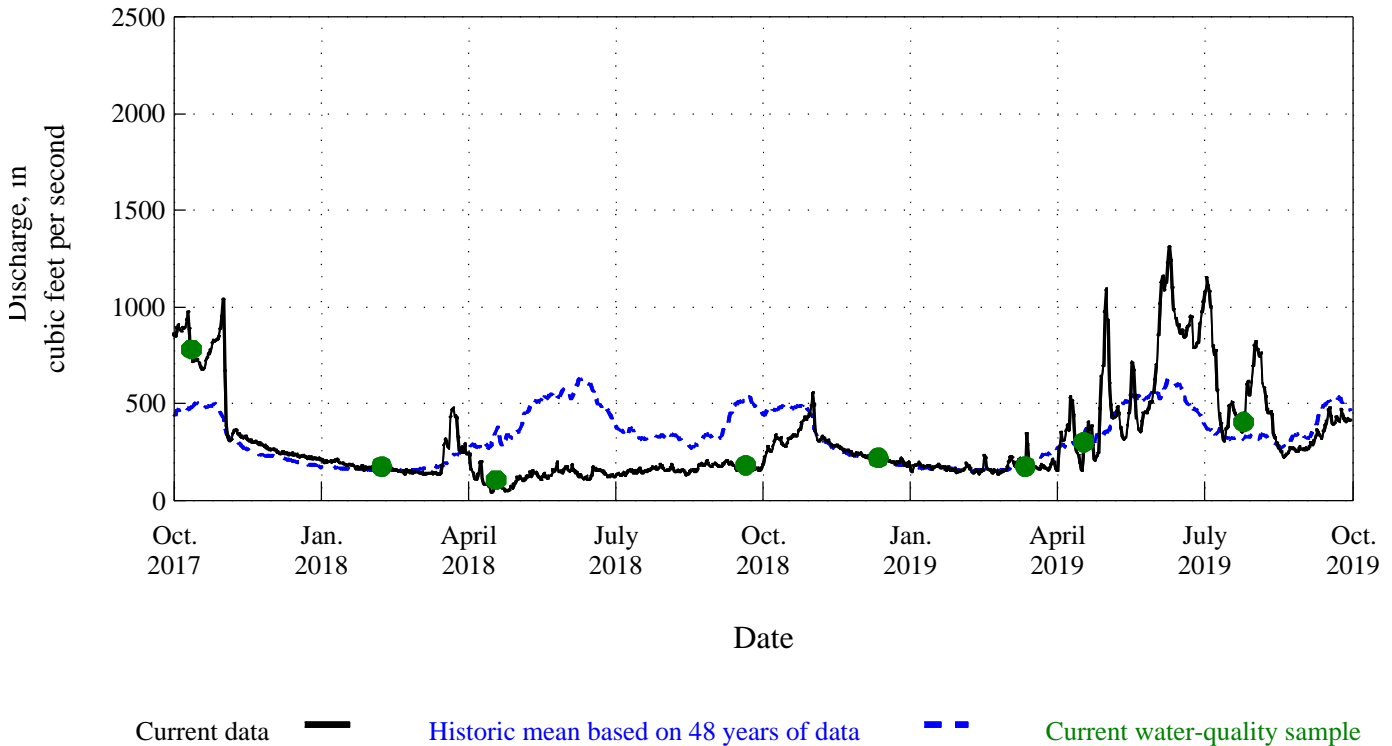
Figure 14. Time distribution and associated discharge of water-quality samples for Uncompahgre River at Delta, CO, station 09149500.
