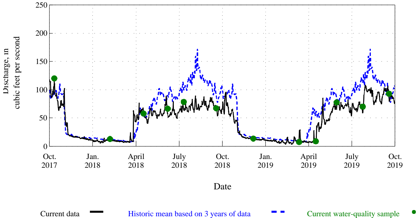
Figure 11. Time distribution and associated discharge of water-quality samples for Loutsenhizer Arroyo below North River Road near Delta, CO, station 383946107595301.
