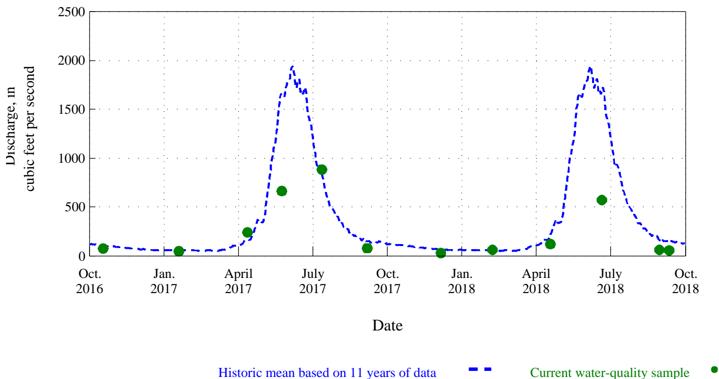
Figure 11. Time distribution and associated discharge of water-quality samples for Eagle River at Avon, Co., station 09067005.
