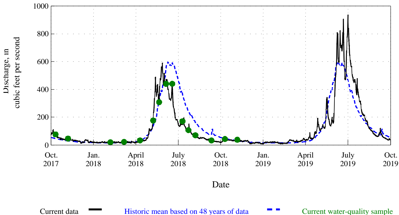
Figure 6. Time distribution and associated discharge of water-quality samples for Big Thompson River at Estes Park, Co., station 06733000.
