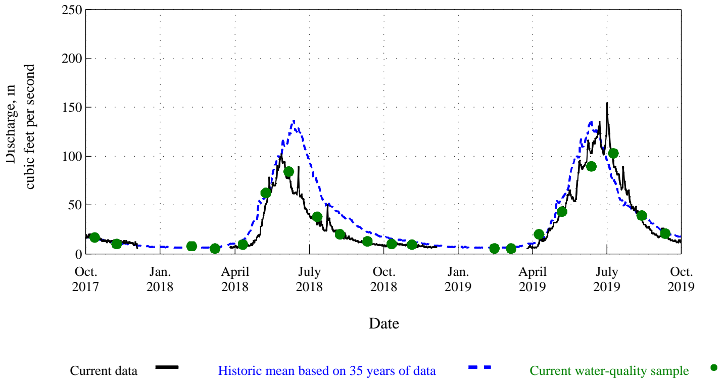
Figure 15. Time distribution and associated discharge of water-quality samples for North Fork Big Thompson River at Drake, Co., station 06736000.
