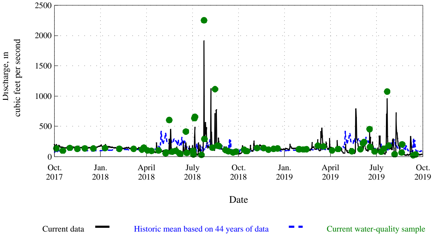
Figure 65. Time distribution and associated discharge of water-quality samples for Fountain Creek near Pinon, Co., station 07106300.
