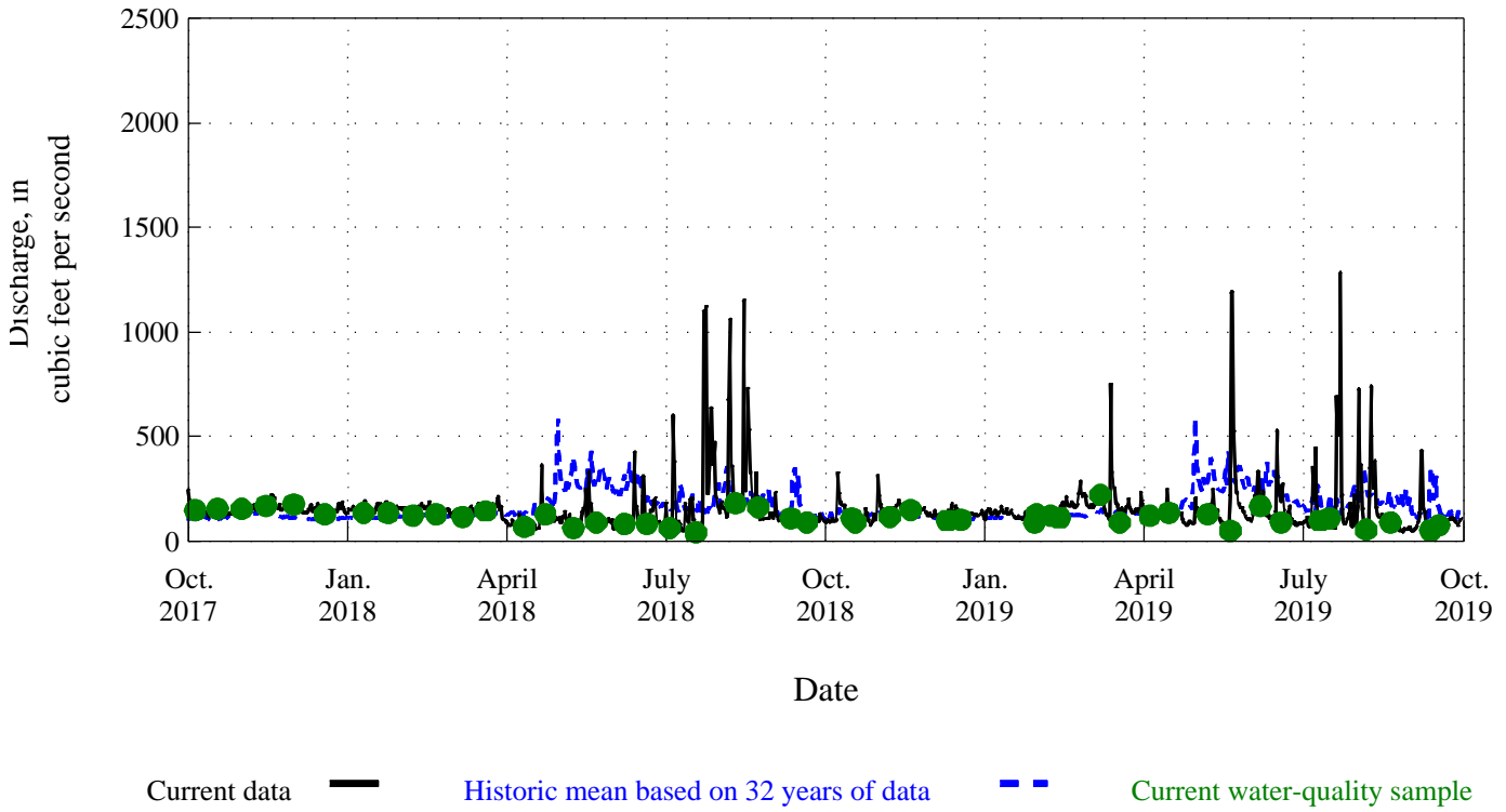
Figure 61. Time distribution and associated discharge of water-quality samples for Fountain Creek near Fountain, Co., station 07106000.
