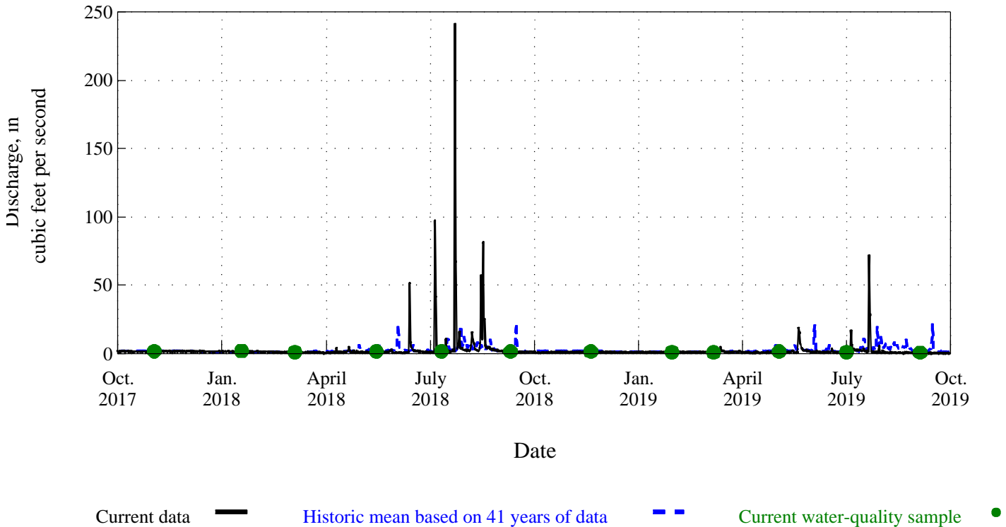
Figure 55. Time distribution and associated discharge of water-quality samples for Jimmy Camp Creek at Fountain, Co., station 07105900.
