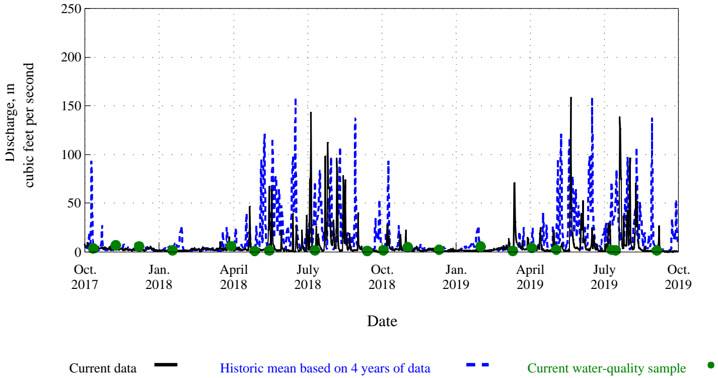
Figure 51. Time distribution and associated discharge of water-quality samples for Sand Creek above mouth at Colorado Springs, Co., station 07105600.
