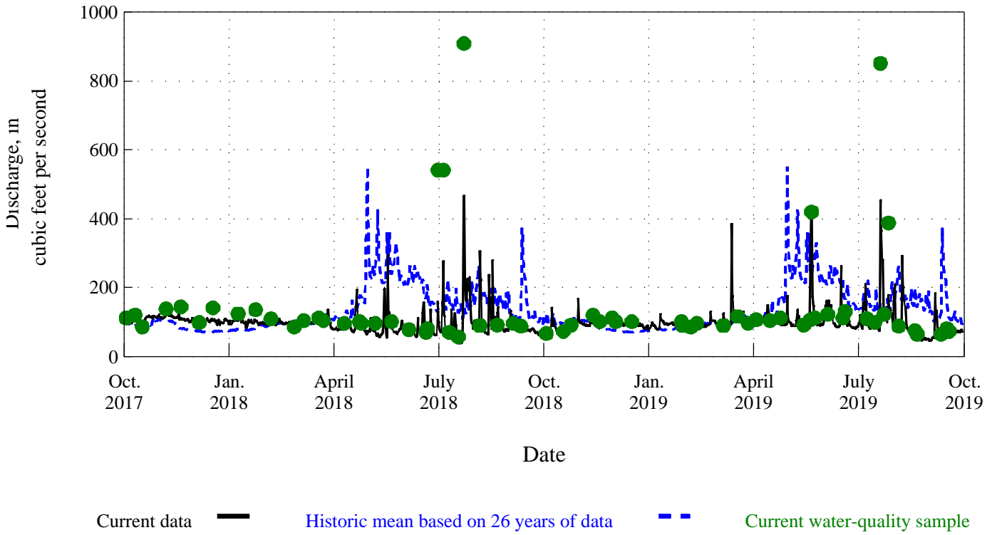
Figure 49. Time distribution and associated discharge of water-quality samples for Fountain Creek below Janitell Rd. below Colorado Springs, Co., station 07105530.
