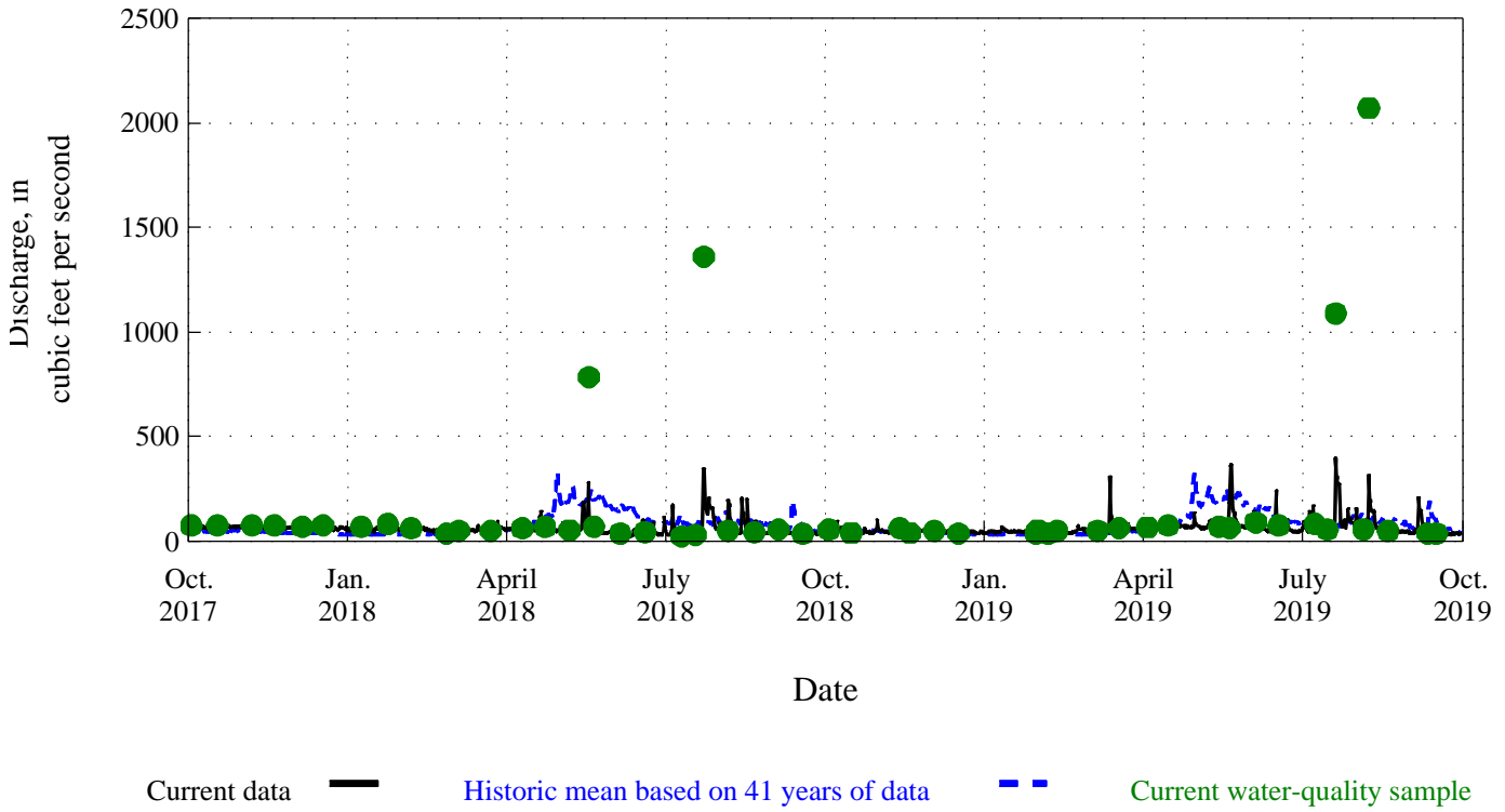
Figure 45. Time distribution and associated discharge of water-quality samples for Fountain Creek at Colorado Springs, Co., station 07105500.
