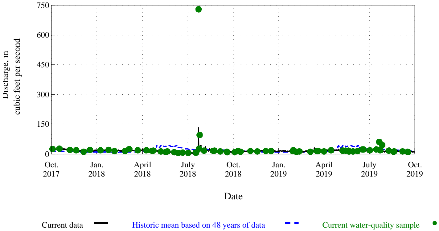
Figure 42. Time distribution and associated discharge of water-quality samples for Fountain Creek near Colorado Springs, Co., station 07103700.
