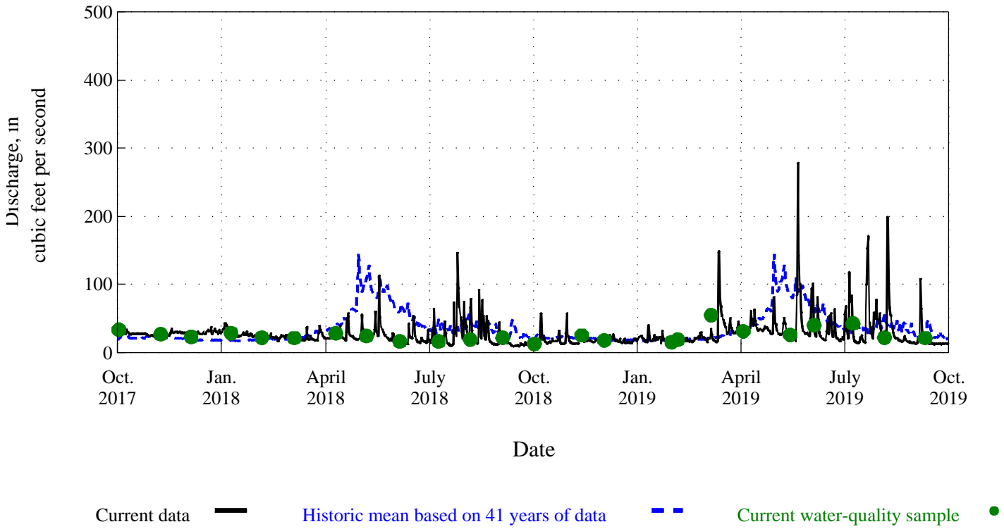
Figure 37. Time distribution and associated discharge of water-quality samples for Monument Creek at Pikeview, Co., station 07104000.
