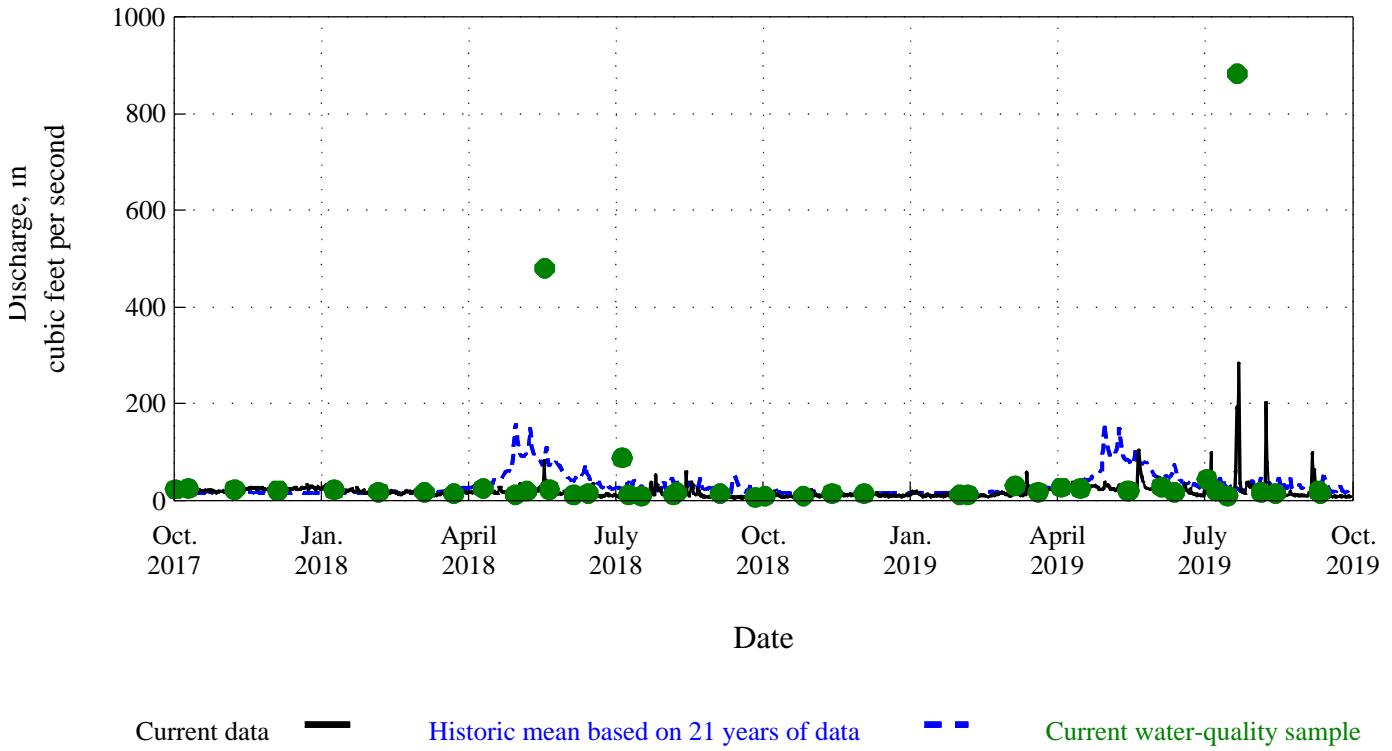
Figure 33. Time distribution and associated discharge of water-quality samples for Monument Creek above Woodmen Road at Colorado Springs, Co., station 07103970.
