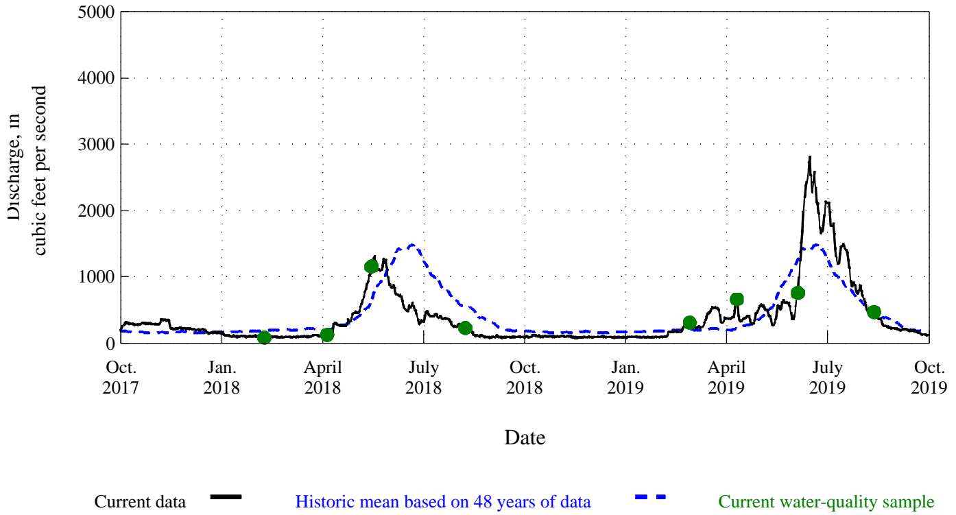
Figure 2. Time distribution and associated discharge of water-quality samples for Arkansas River at Granite, Co. (ARKGRNCO), station 07086000.
