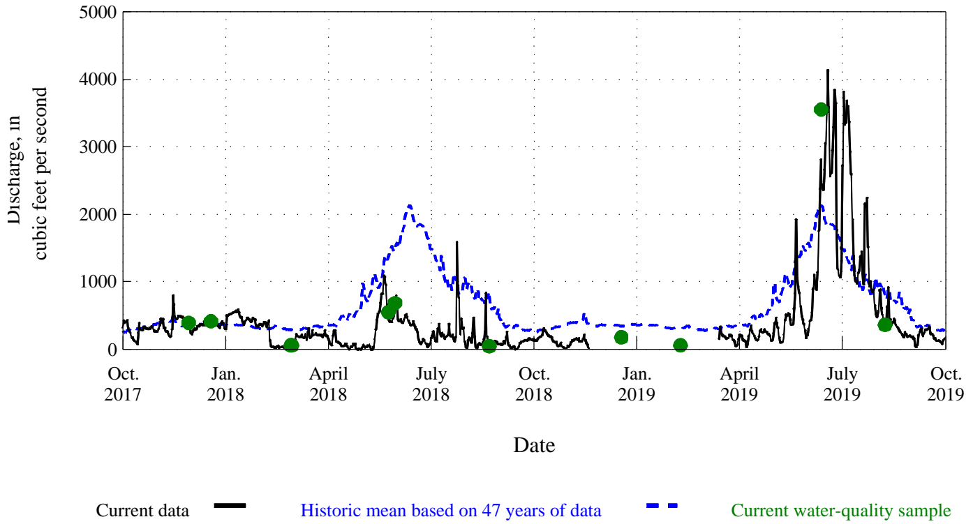
Figure 17. Time distribution and associated discharge of water-quality samples for Arkansas River at Catlin Dam near Fowler, Co. (ARKCATCO), station 07119700.
