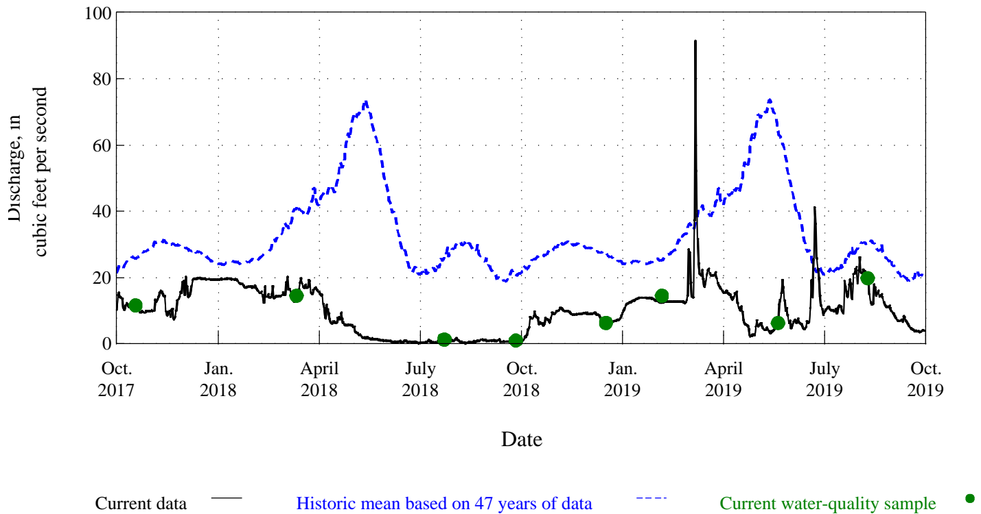
Figure 4. Time distribution and associated discharge of water-quality samples for Piceance Creek at White River, Co., station 09306222.
