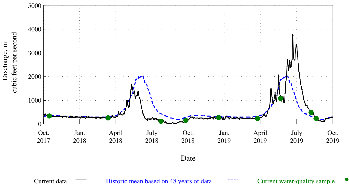
Figure 15. Time distribution and associated discharge of water-quality samples for White River above Coal Creek, near Meeker, Co., station 09304200.
