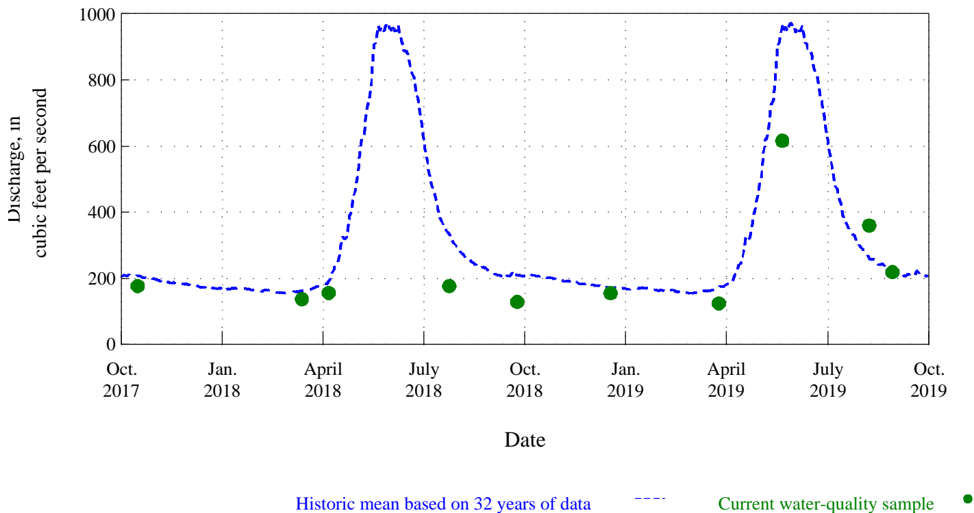
Figure 10. Time distribution and associated discharge of water-quality samples for North Fork White River at Buford, Co., station 09303000.
