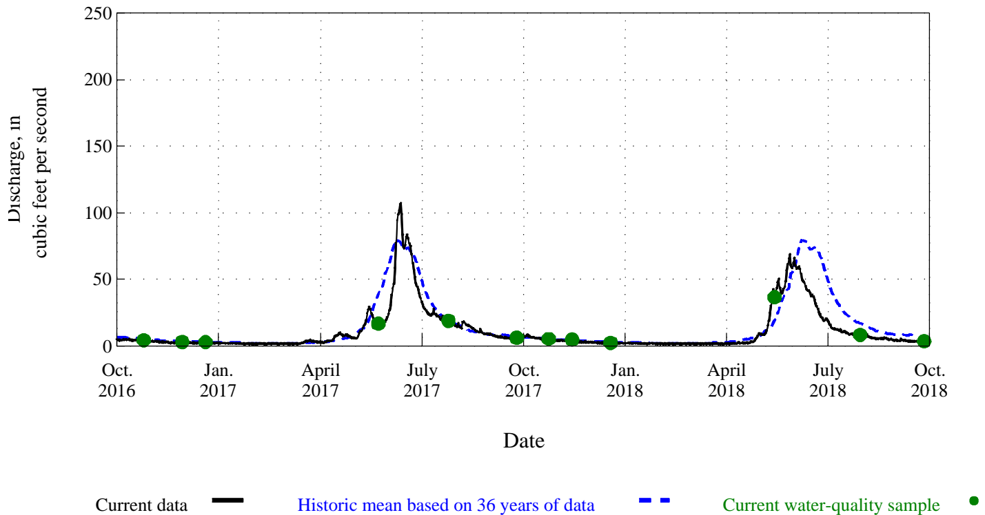
Figure 2. Time distribution and associated discharge of water-quality samples for Fraser River at Upper Station, near Winter Park, CO., station 09022000.
