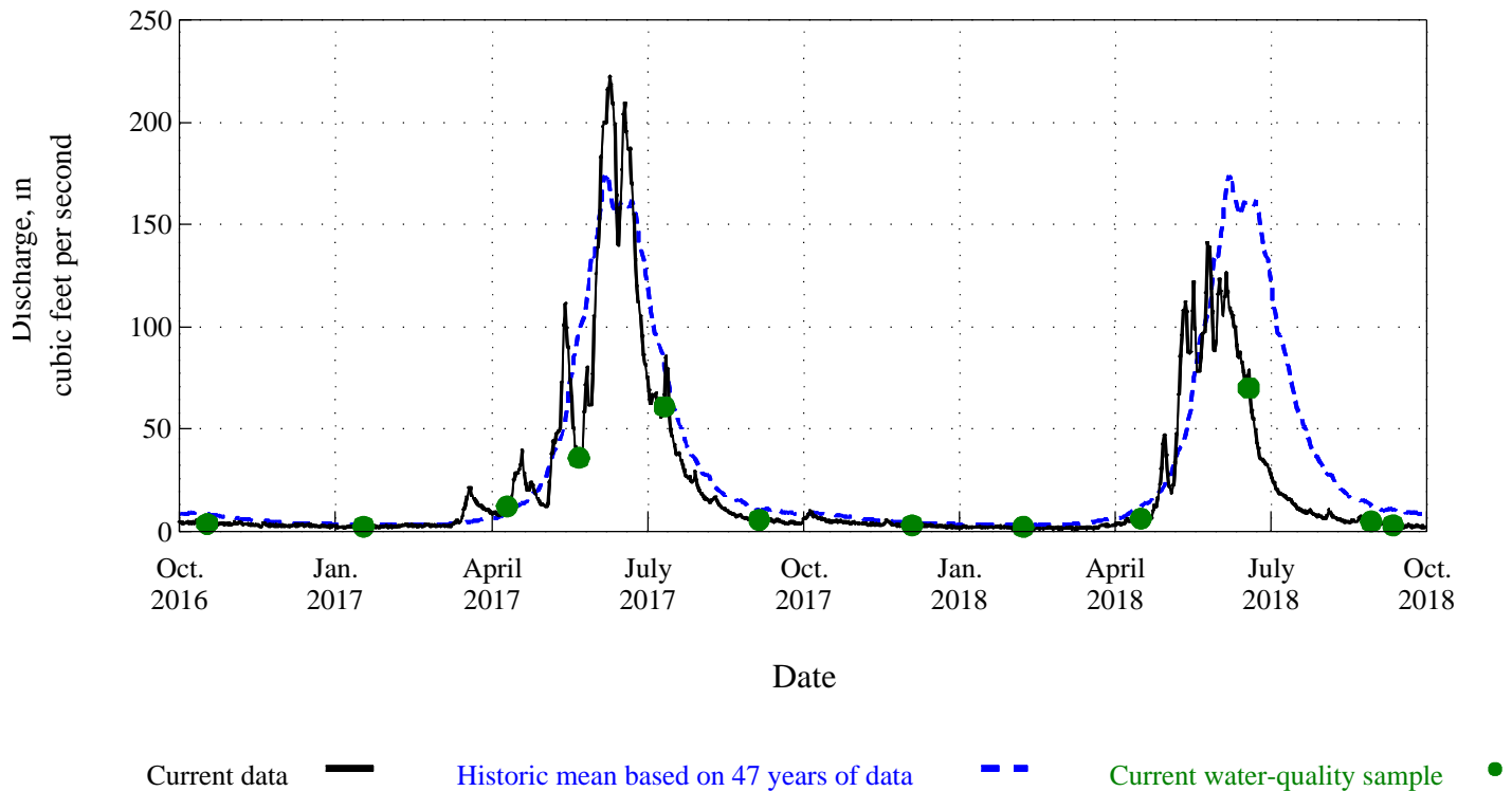
Figure 2. Time distribution and associated discharge of water-quality samples for Gore Creek at Upper Station, near Minturn, Co., station 09065500.
