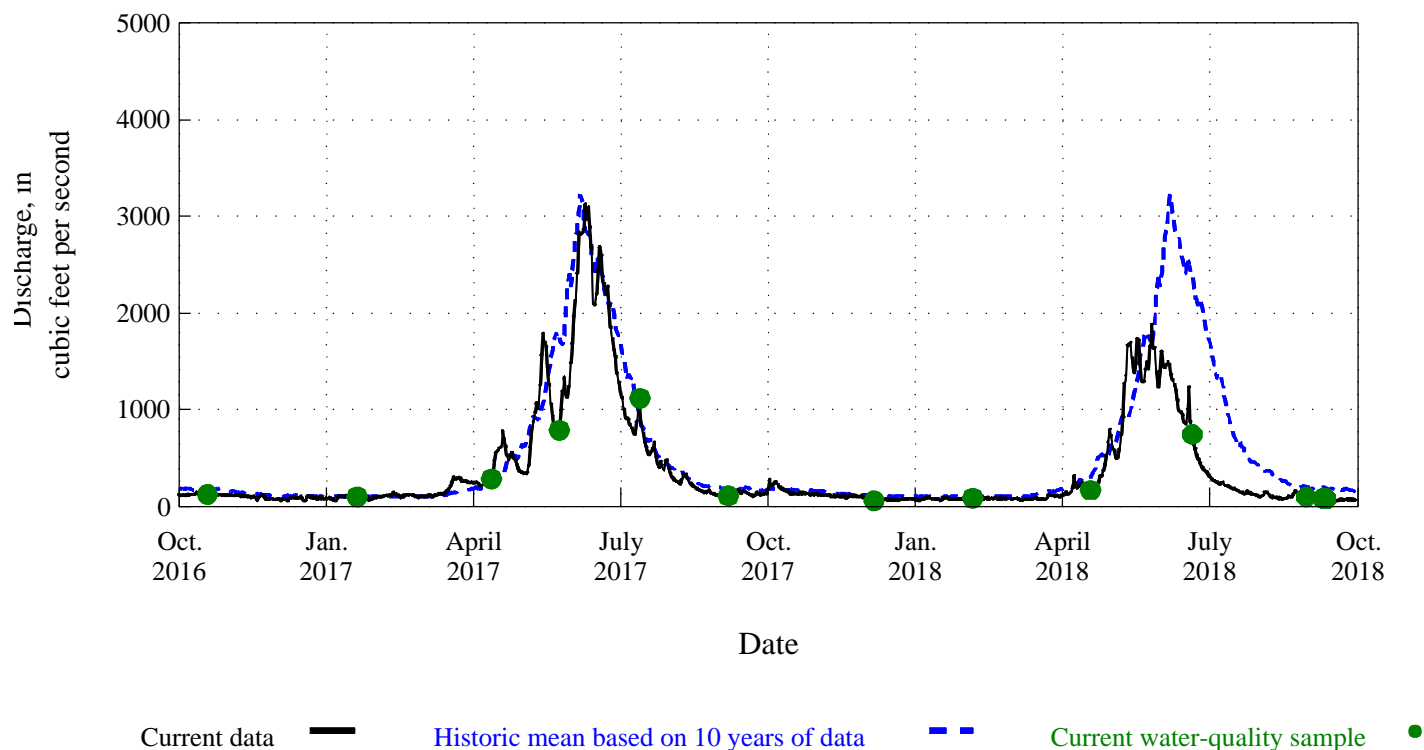
Figure 13. Time distribution and associated discharge of water-quality samples for Eagle River below Milk Creek, near Wolcott, Co., station 394220106431500.
