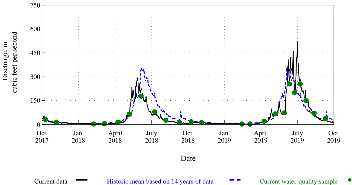
Figure 4. Time distribution and associated discharge of water-quality samples for Big Thompson River below Moraine Park, station 402114105350101.
