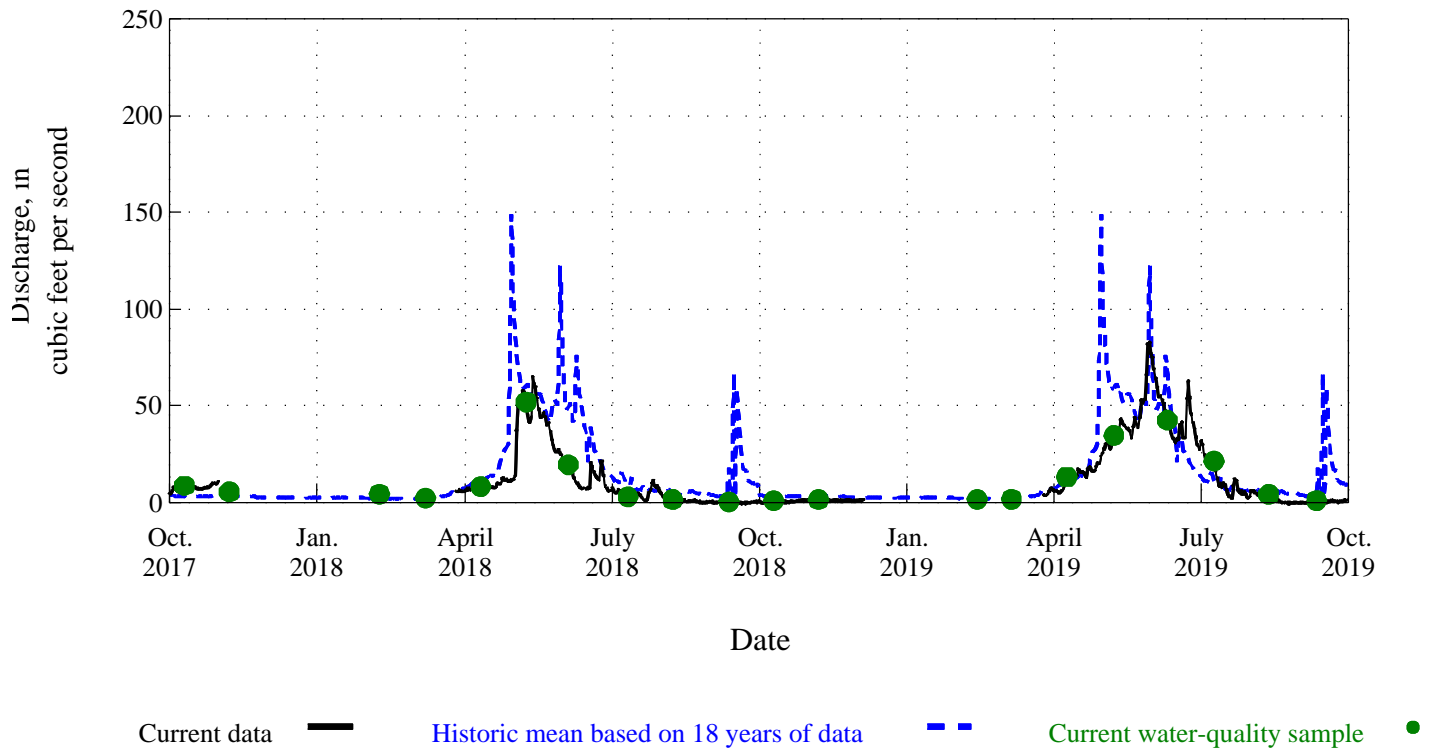
Figure 20. Time distribution and associated discharge of water-quality samples for Buckhorn Creek near Masonville, Co., station 06739500.
