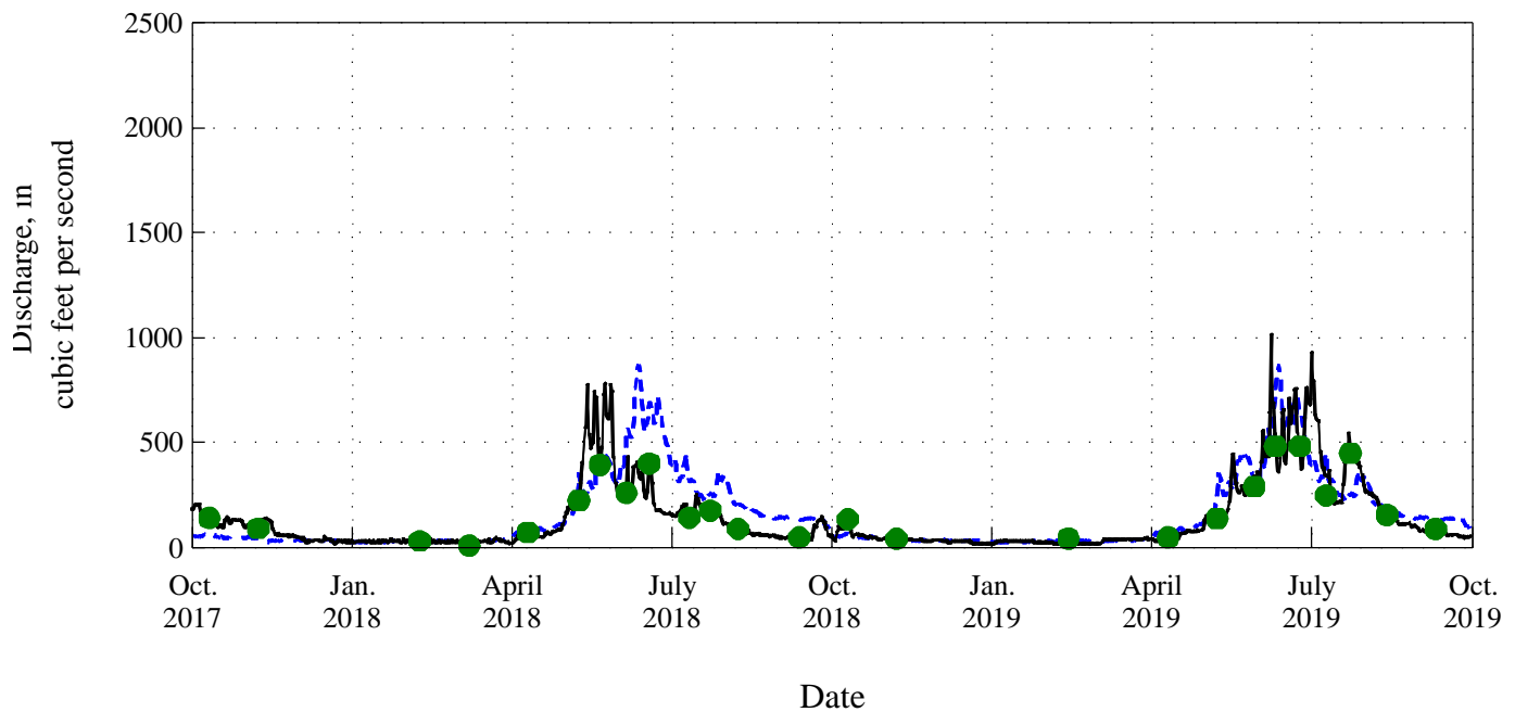
Figure 17. Time distribution and associated discharge of water-quality samples for Big Thompson River above Dille Tunnel, near Drake, Co., station 06736700.
