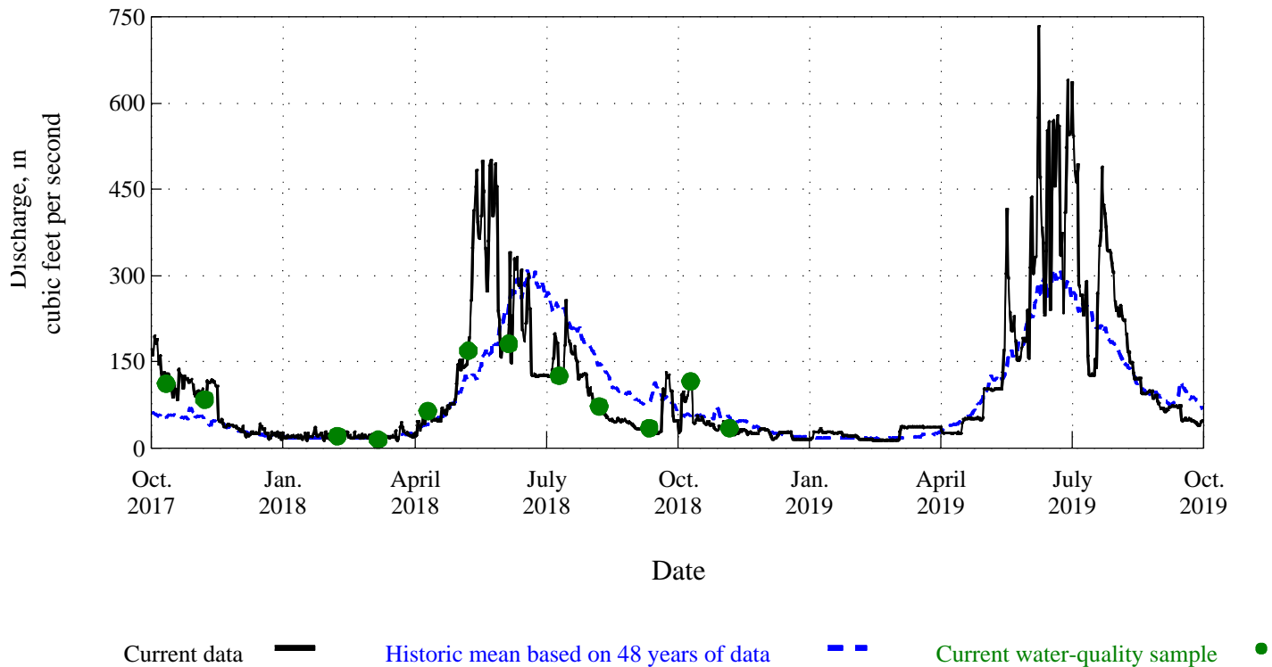
Figure 11. Time distribution and associated discharge of water-quality samples for Big Thompson River near Estes Park, Co., station 06735500.
